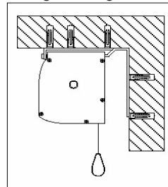
Ceiling Mounting
