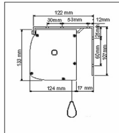
Cabinet dimensions
